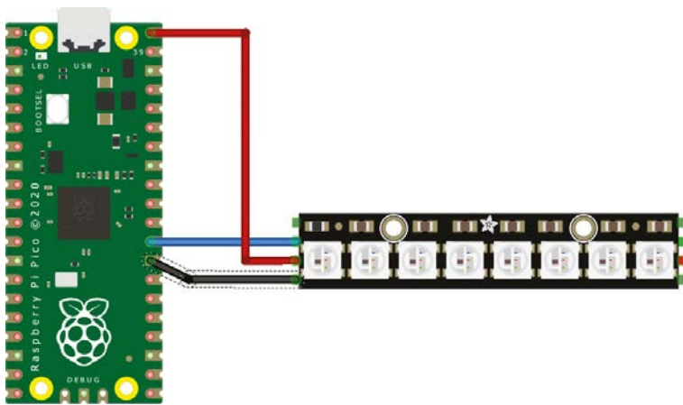
▲ Figure 1: Pin 40 (top-right) is the 5v pin, while every square pin on Pico is ground
